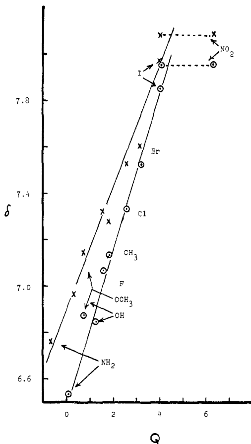
Figure 3. Plot of the H-3 chemical shifts for the 2-X-acetophenones vs. Q . The lower line is for carbon tetrachloride solutions and the upper is for DMSO.
